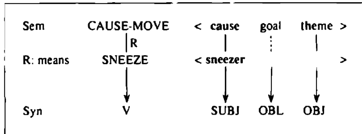
Composite Structure: Caused-Motion + sneeze :
