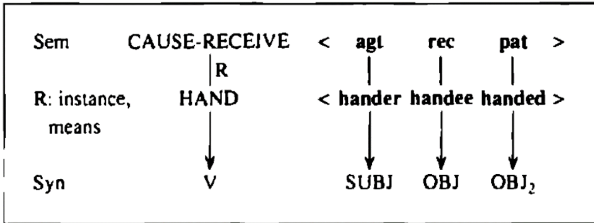
Composite Fused Structure: Diransitive + hand
