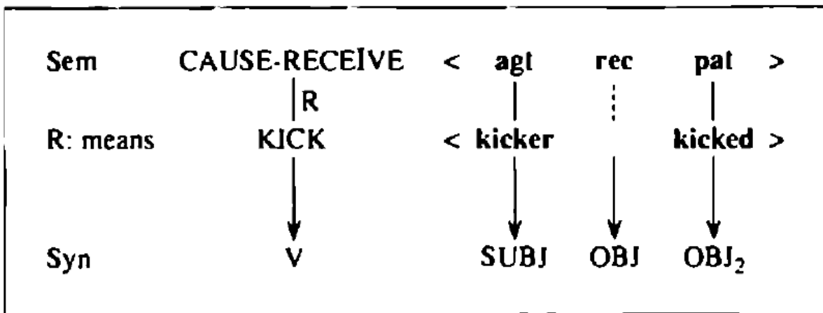
Composite Structure: Ditransitive + kick :
